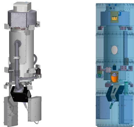
Figure 9. X-ray radiography facility MIDAS-M with sample chamber (top), X-ray tube, and ion-getter pump (bottom).
