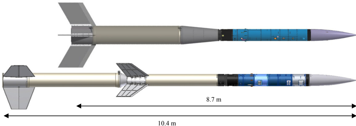
Figure 10. The MAPHEUS-4 (top) and MAPHEUS-3 (bottom) vehicles with motor(s), motor adapter and payload sections (blue).
