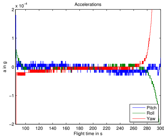
Figure 8. Accelerations in three axes after activation of the rate-control system.
