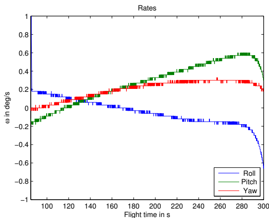
Figure 11. Residual rates after rate-control system activation.
