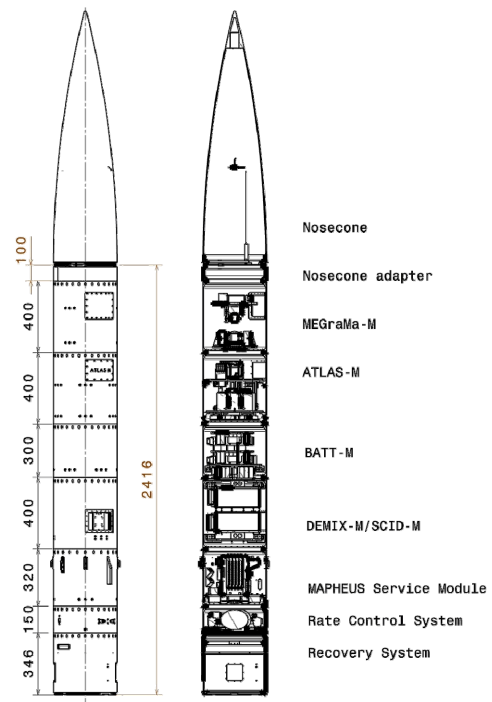
Figure 7. Overview of the MAPHEUS-3 payload stack
